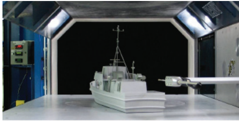
FIGURE 6. 4% scale YP model in USNA wind tunnel.
