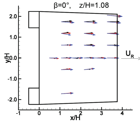
FIGURE 13. Horizontal vertical plane z/H=1.08 (63.7 inches) above the flight deck for a headwind (black arrows are in situ data, red arrows are wind tunnel data, and blue arrows are CFD data).
