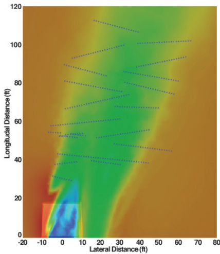
FIGURE 18. Measured air wake location (blue dashed lines) and CFD simulation (colored background) for \beta=30^\circ at the top of the hangar structure.
