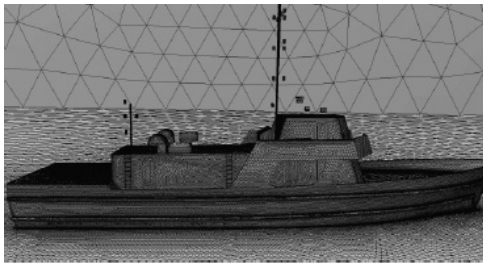
FIGURE 7. Unstructured surface grid.
