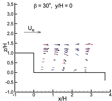
FIGURE 12. Centerline vertical plane ( y/H=0 ) for relative wind \beta=30^\circ (black arrows are in situ data, red arrows are wind tunnel data, and blue arrows are CFD data).
