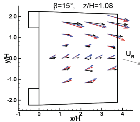
FIGURE 14. Horizontal vertical plane z/H=1.08 (63.7 inches) above the flight deck for relative wind \beta=15^\circ (black arrows are in situ data, red arrows are wind tunnel data, and blue arrows are CFD data).
