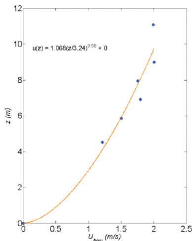
FIGURE 20. Atmospheric boundary layer observed during May 2012 underway testing. A least squares fit of horizontal velocity, less ship velocity U_{YP} , is shown.
