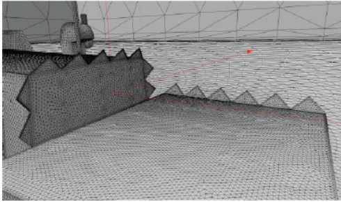
FIGURE 22. CFD grid showing flow control fences added to the top, port, and starboard sides of hangar structure and starboard side of flight deck.
