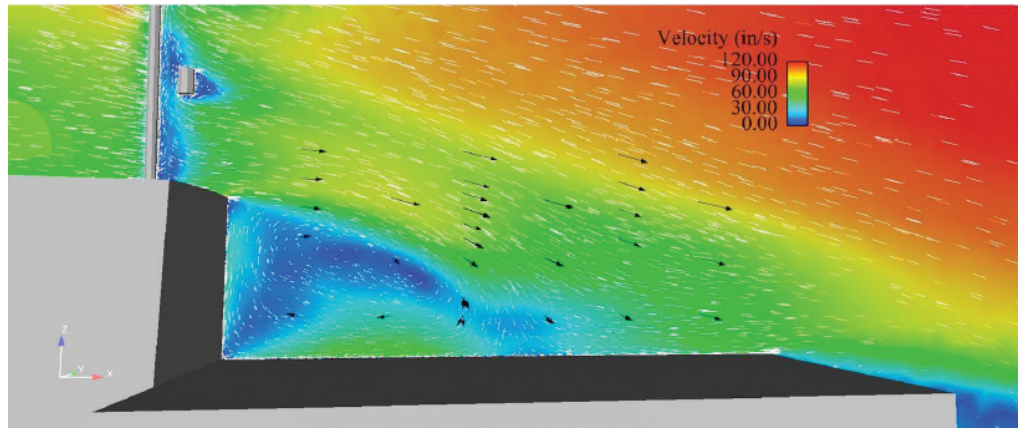
FIGURE 8. Scaled in situ data (black arrows) vs. 7 knot CFD simulations (white arrows and color contours) for headwind ( \beta=0^\circ ) at centerline of the flight deck (7 knots=141 in/s). Locations with multiple black arrows are where data were taken on different days.
