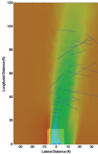
FIGURE 17. Measured air wake location (blue dashed lines) and CFD simulation (colored background) for \beta=15^\circ at the top of the hangar structure.
