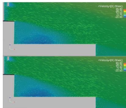
FIGURE 21. Comparison of CFD simulations for \beta=0^\circ . Top is grid with 17 million tetrahedral while bottom is grid with 22 million tetrahedral.
