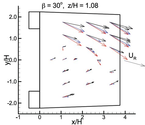
FIGURE 15. Horizontal vertical plane z/H=1.08 (63.7 inches) above the flight deck for relative wind \beta=30^\circ (black arrows are in situ data, red arrows are wind tunnel data, and blue arrows are CFD data).
