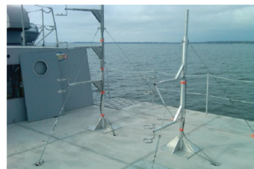
FIGURE 4. Ultrasonic anemometers installed on YP676 flight deck.
