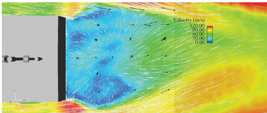
FIGURE 9. Scaled in situ (black arrows) vs. 7 knot CFD simulations (white arrows and color contours) for relative wind \beta=15^\circ for the horizontal plane 17 inches above the flight deck (7 knots=141 in/s). Locations with multiple black arrows are where data were taken on different days.
