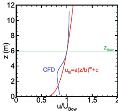
FIGURE 19. Fitted power law velocity profile (red line) of underway anemometer data vs. CFD velocity profile (blue line). The green line is the height of the bow reference anemometer. ( a , b , c , and m are constants determined through least-square curve fitting, z is the distance above the vessel’s waterline, and u_{fit} is the fitted velocity.)
